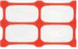
Material: LDPE/HDPE/U.V. Mesh Size: 80mm*40mm Weight: 140-200gram Width(Diameter): 1m/1.22m Colors: orange/green/yellow
