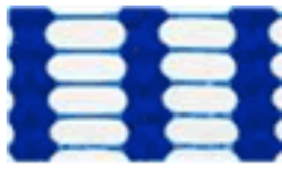
Material: LDPE/HDPE/U.V. Mesh Size: 80mm*26mm Weight: 280gram
