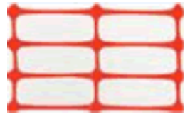
Material: LDPE/HDPE/U.V. Mesh Size: 100mm*40mm Weight: 80-120gram Width(Diameter): 1m/1.22m Colors: orange/green/yellow
